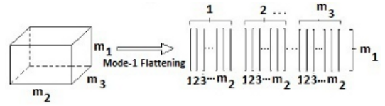
Fig. 1. Mode-1 flattening operation for third-order tensors (Source: Adapted from [4]).
